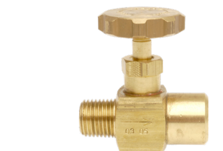
NV404/808 Male and Female Needle Valve
